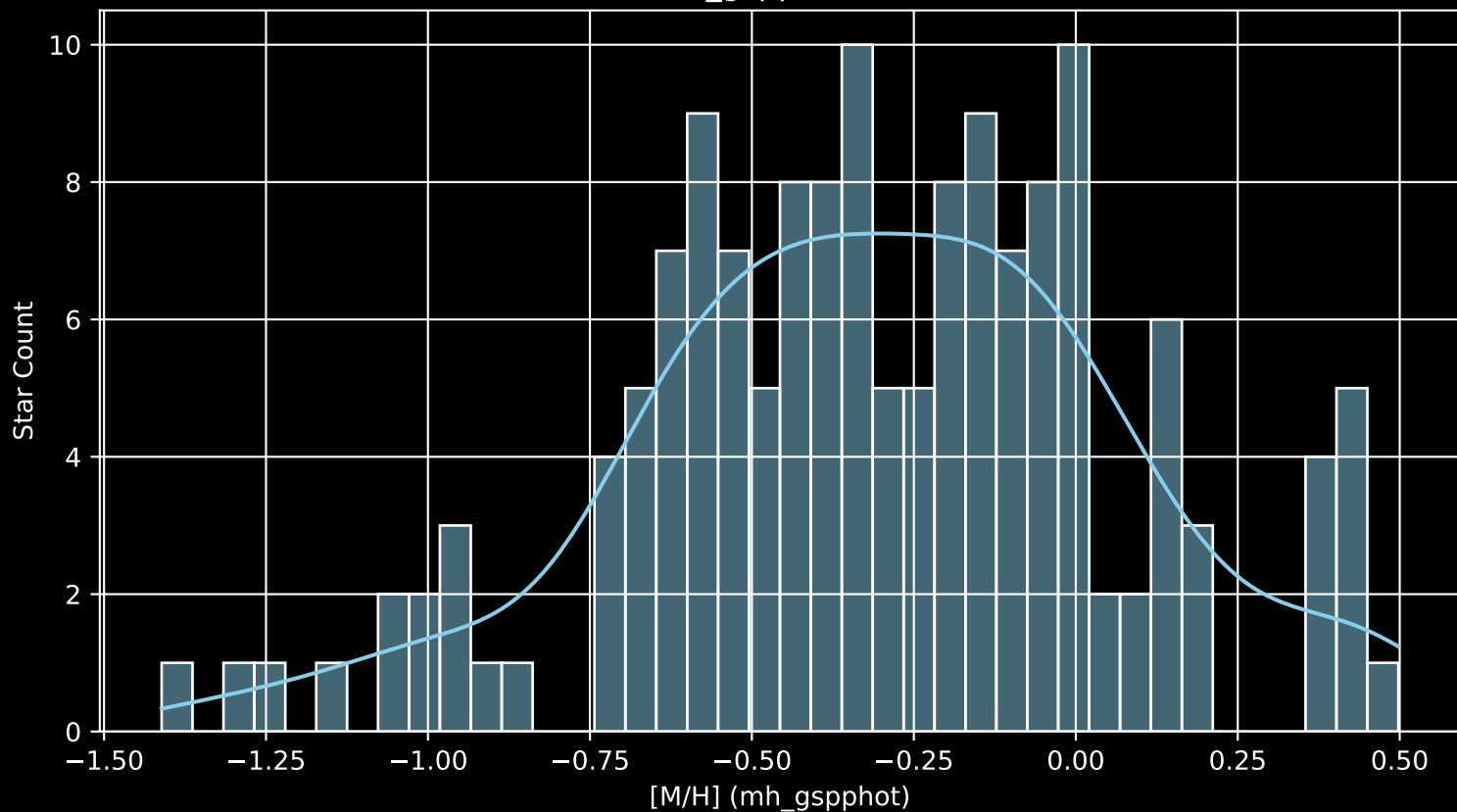
APOGEE DR17 Field: [355+23-O [M/H] (mh_gspphot) (n= 151)
