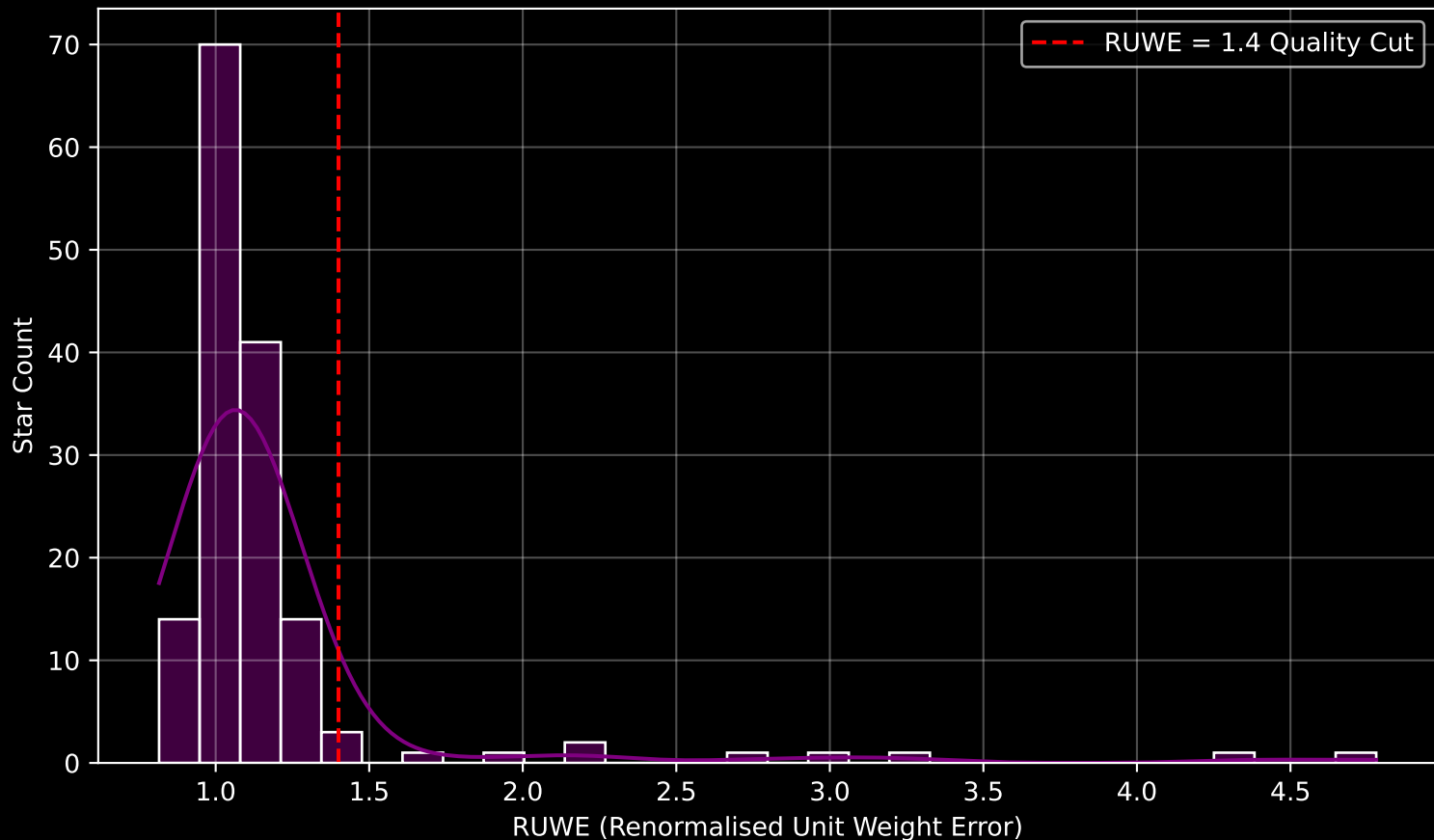
GAPOGEE DR17 Field [355+23-O] RUWE Distribution (n= 151)
