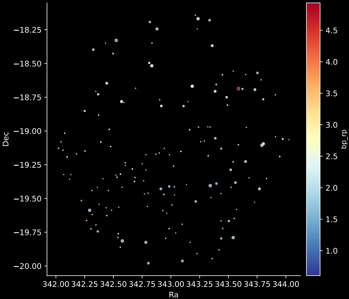
APOGEE DR17 Field: [355+23-O] Stars: 154
