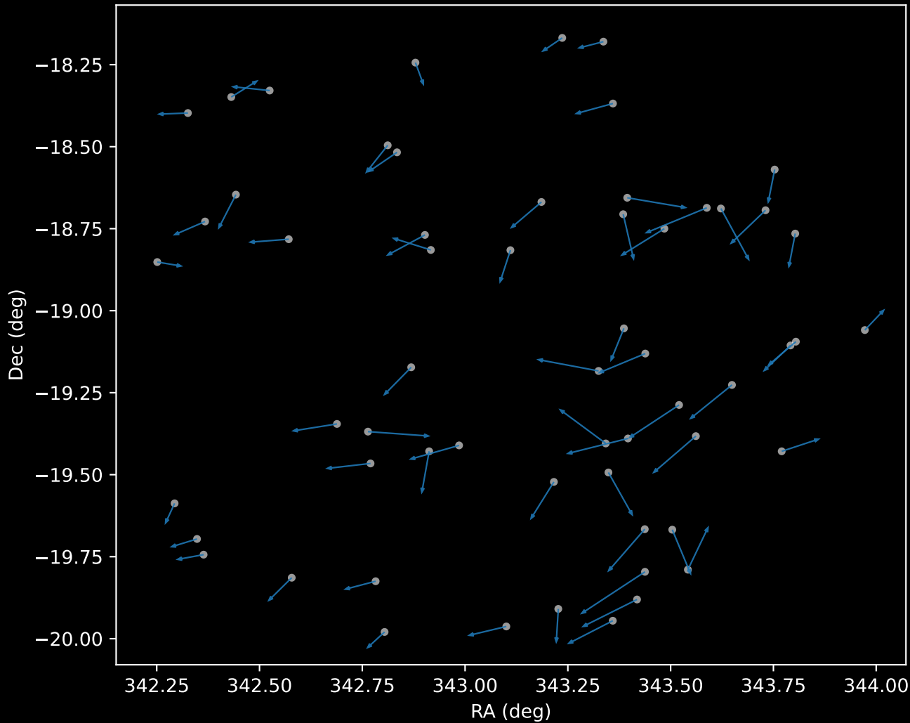
APOGEE DR17 Cluster 0 Proper Motion Vectors (n=59)
