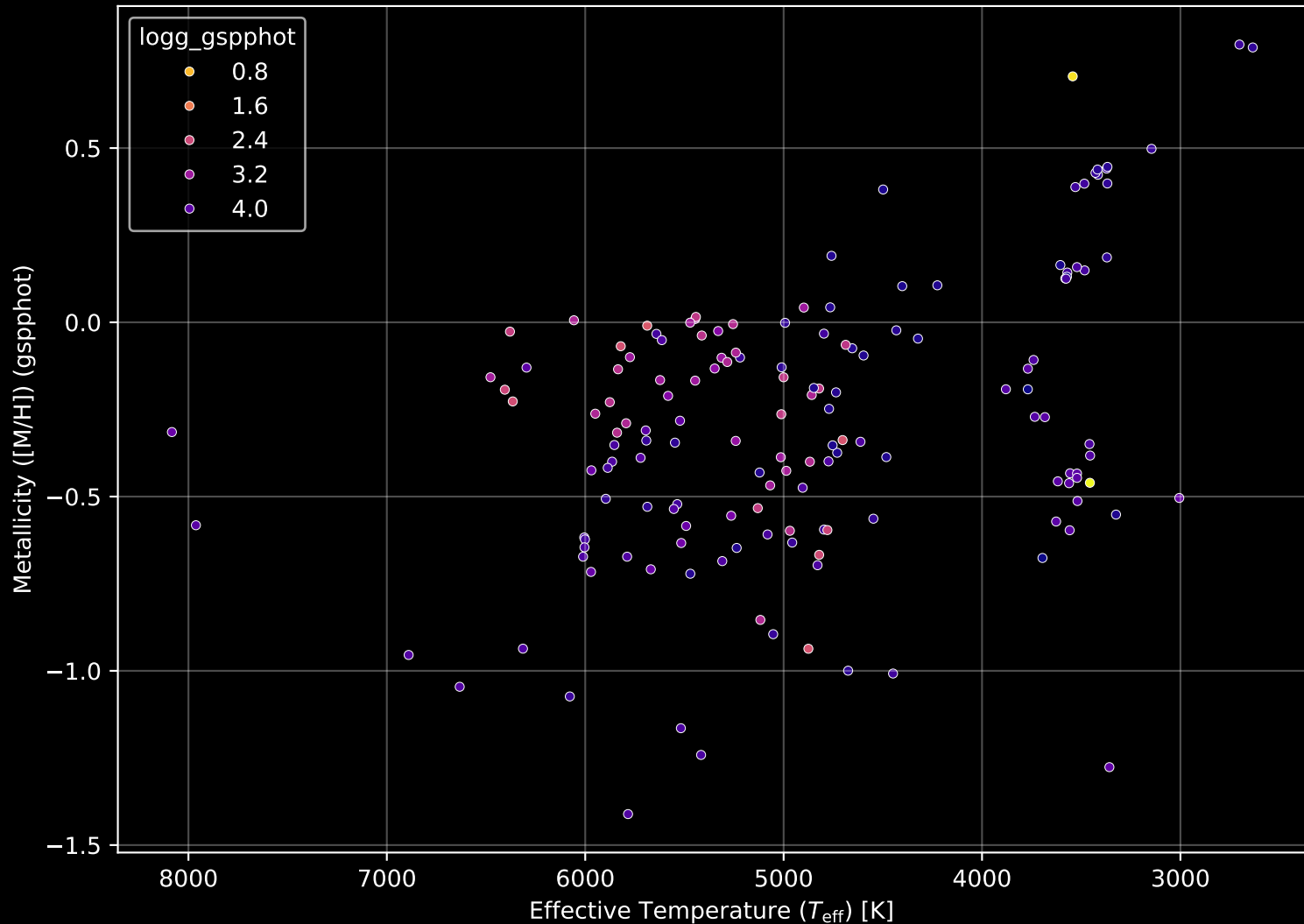
APOGEE DR17 Field: [355+23-O] Stellar Population Parameters (n= 154)
