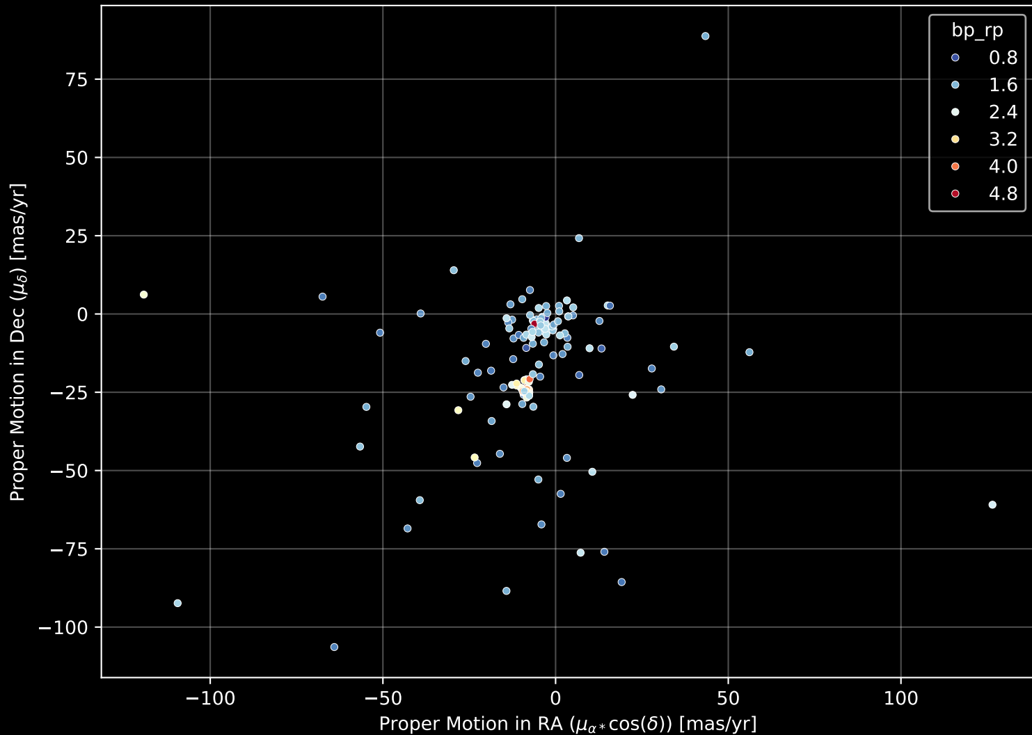
APOGEE DR17 Field: [355+23-O] Proper Motion Diagram (n= 154)
