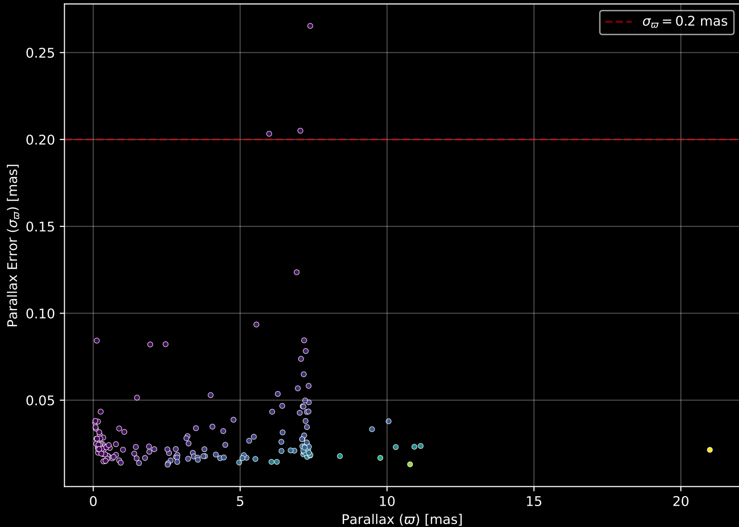
APOGEE DR17 Field: [355+23-O] Parallax Quality (n= 154)
