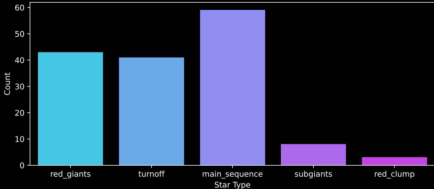
APOGEE DR17 Field: [355+23-O] Count plot of Star Type
